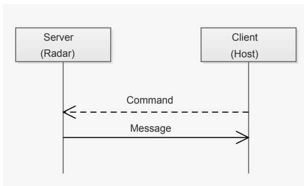
Figure 11: Client-Server model
