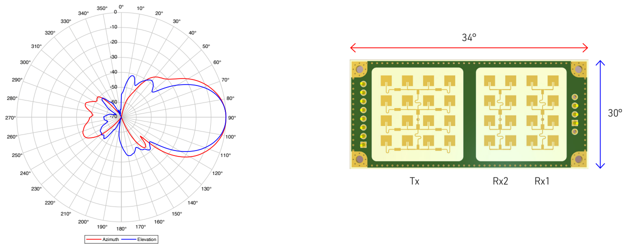
Figure 2: Overall antenna diagram
