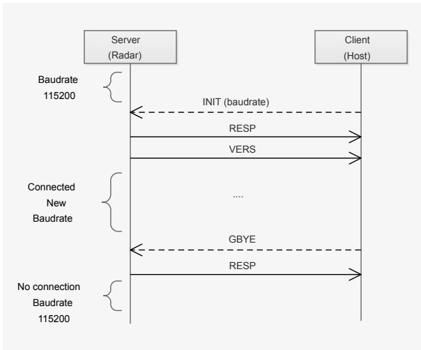
Figure 13: Connection
