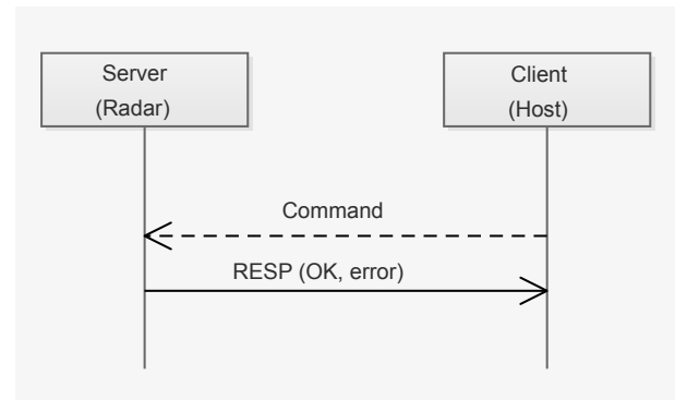
Figure 12: Handshaking
