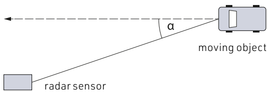
Figure 5: Tangential speed compensation
