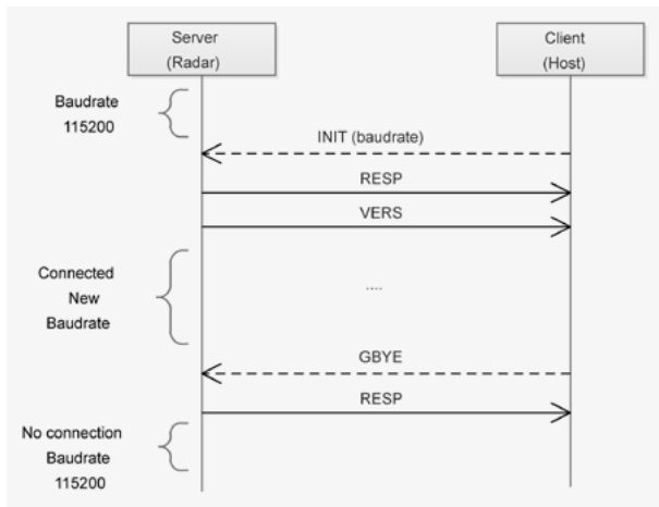
Figure 11: Connection
