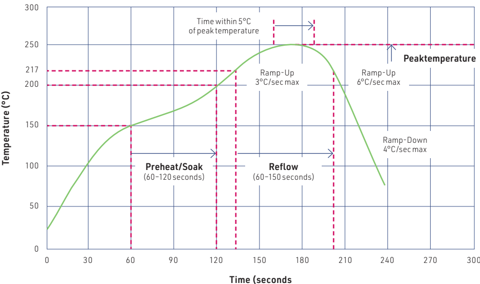
Figure 23: Typical reflow profile
