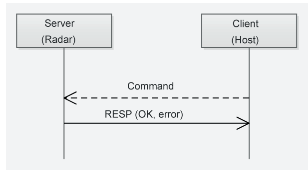
Figure 10: Handshaking
