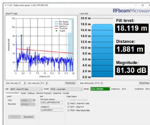
Figure 1: Control panel
