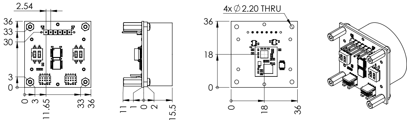
Figure 14: Outline dimensions in millimetre
