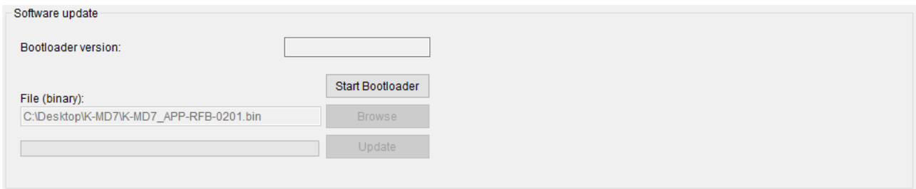
Figure 13: Update tab
