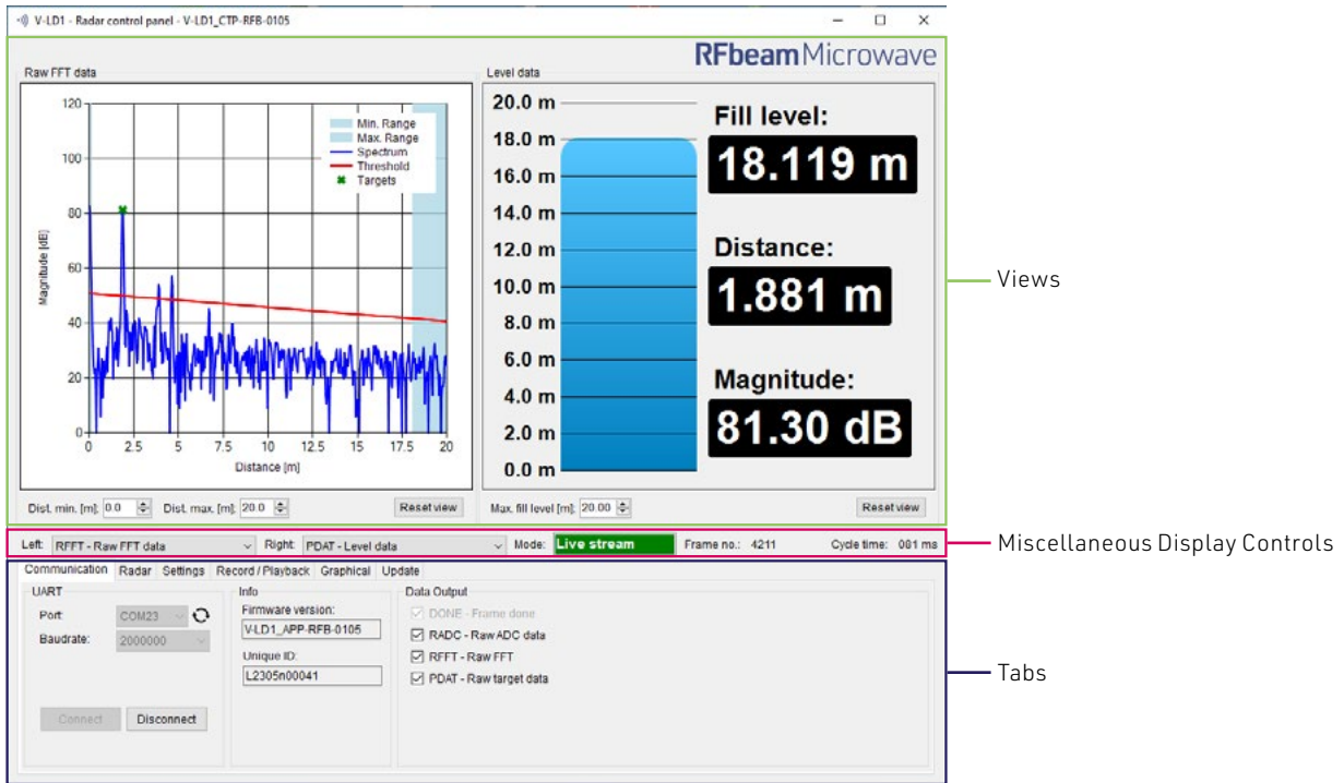
Figure 5: Overview control panel areas
