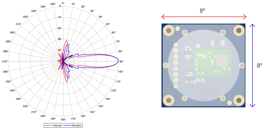
Figure 3: Overall antenna diagram with lens
