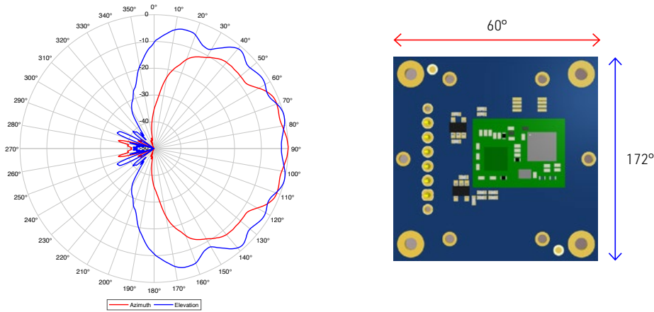
Figure 2: Overall antenna diagram without lens
