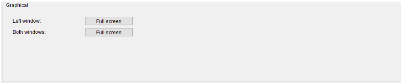
Figure 12: Graphical tab
