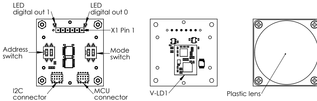
Figure 4: Pin configuration and functions
